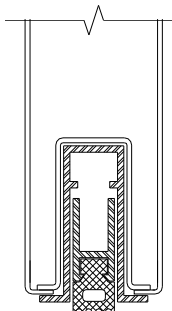
Door Bottom Detail (Varies with manufacturer)
